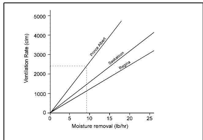
Figure 3. Moisture removal and ventilation rates for daytime conditions.
