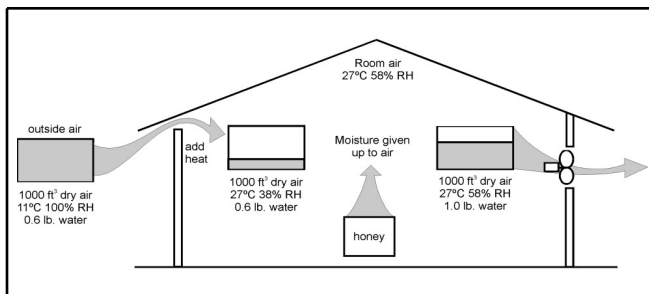
Figure 4. July nighttime conditions for Prince Albert.
