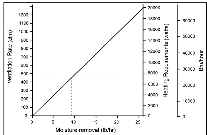
Figure 5. Ventilation rates required and the amount of heat that must be added for moisture removal for night conditions in Saskatchewan.
