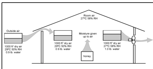
Figure 2. July daytime conditions for Prince Albert.
