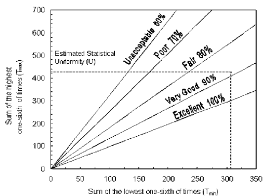
Figure 1. Microirrigation Uniformity Nomograph
