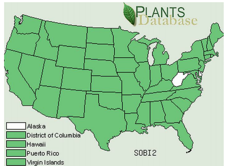
Figure 1. Occurrence of Sorghum bicolor in the U.S.
