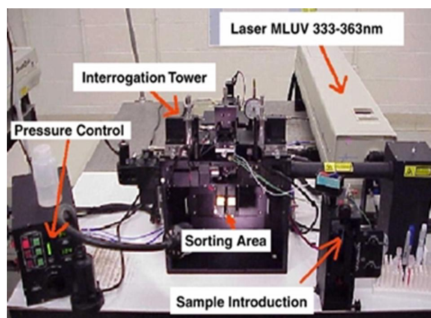
Figure 2. MoFlo® flow cytometer/cell sorter
