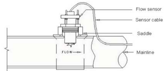
Figure 10. Paddle wheel flow sensor installed in mainline allowing remote monitoring of flow rate in system.
