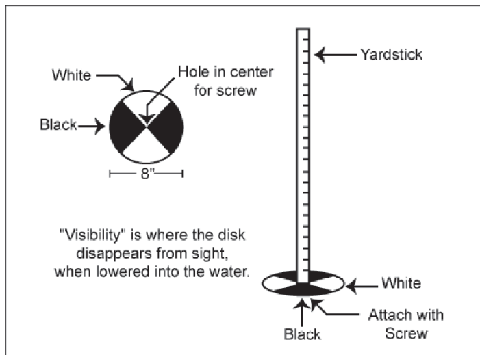
Figure 1. A visibility measurement stick (Secchi disk).
