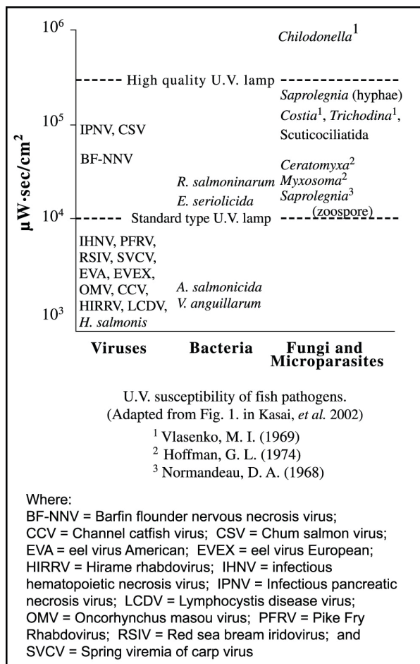
Figure 1. Recommended zap doses for different organisms.
