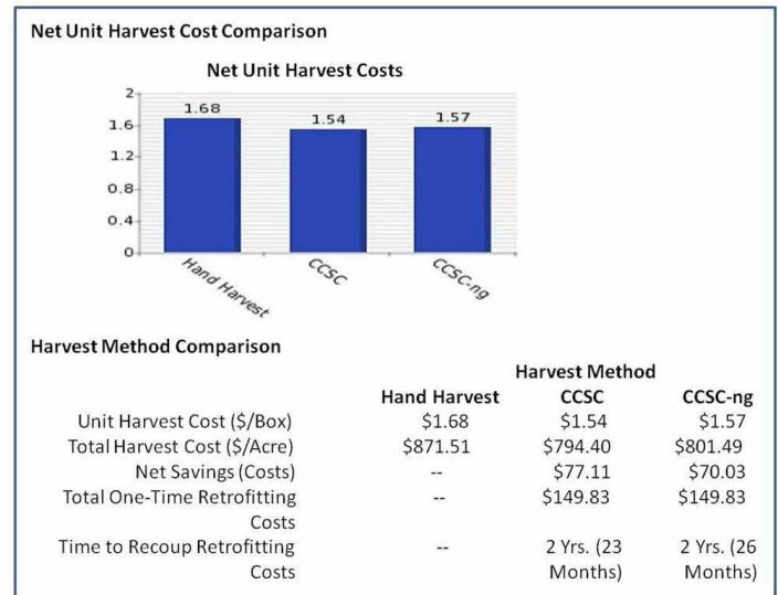
Figure 5. Summary of unit harvesting cost by harvest method.
