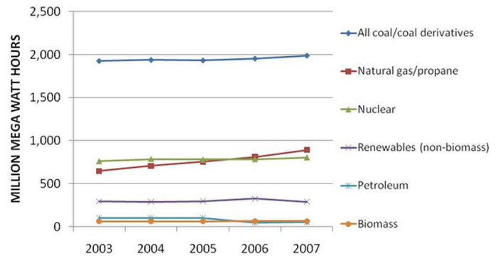
Figure 1. Net electricity generation by U.S. power plants by major fuel groups, 2003–2007.
