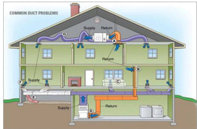
Figure 1. Common Air Duct Problems: A= Leaky connections; B= Leaky return; C= Furniture blocking registers; D= Leaks at furnace and air filter slot and duct tape failures; E=Fallen duct insulation; F=Leaky Supply Ducts; G= Kinks restricting airflow Credits: ENERGY STAR
