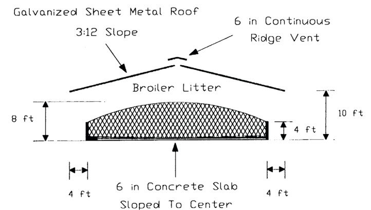
Figure 1. Covered slab.
