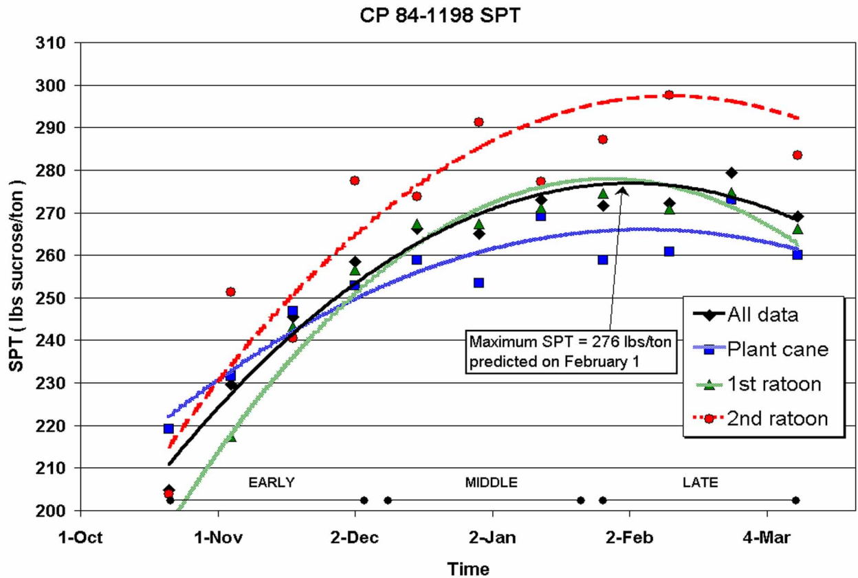
Figure 1. Sucrose Accumulation Maturity Curves for CP 84-1198.
