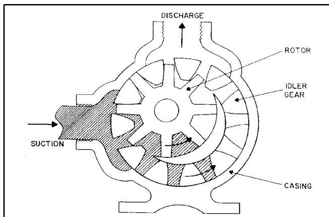
Fig. 4. Internal gear pump.
