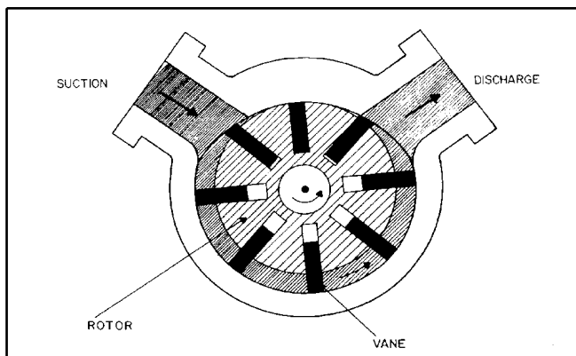
Fig. 7. Vane pump.
