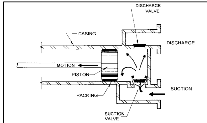
Fig. 2a. Piston pump - suction stroke.
