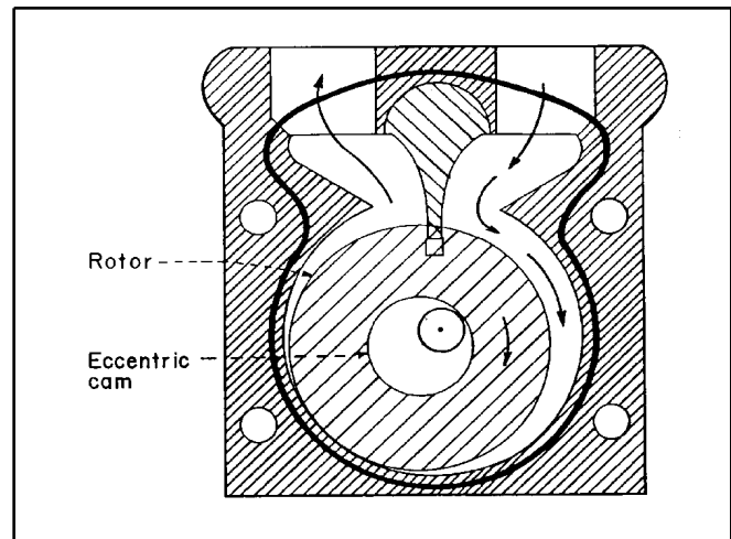
Fig. 10. Eccentric cam pump.
