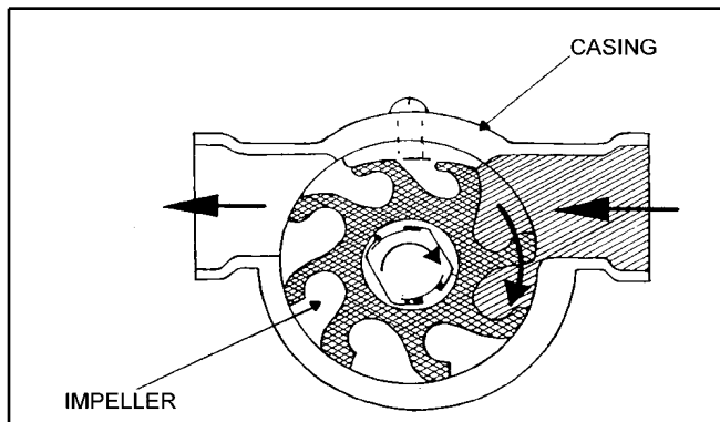
Fig. 9. Flexible impeller pump.
