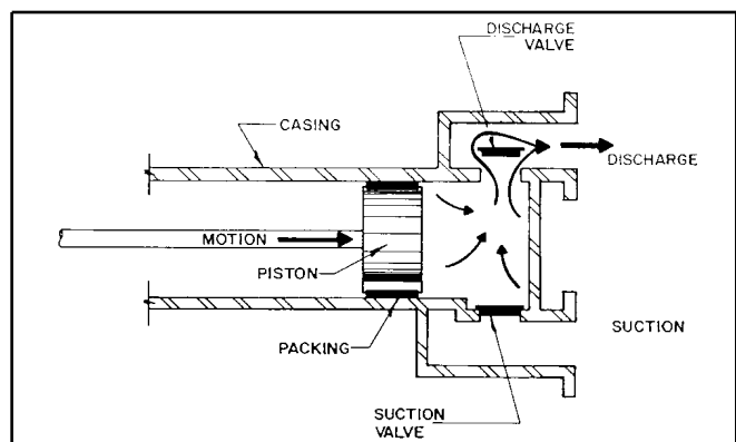
Fig. 2b. Piston pump - discharge stroke.
