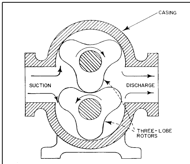
Fig. 6. Lobe pump with two impellers.
