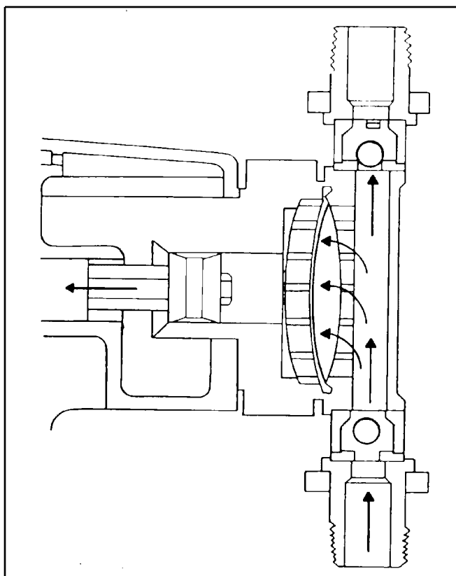
Fig. 3b. Diaphragm pump - discharge stroke.
