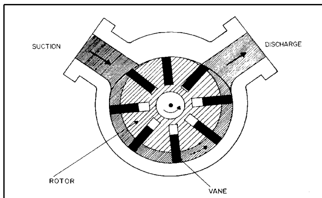
Fig. 7. Vane pump.
