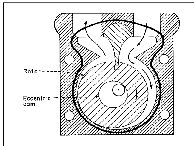
Fig. 10. Eccentric cam pump.
