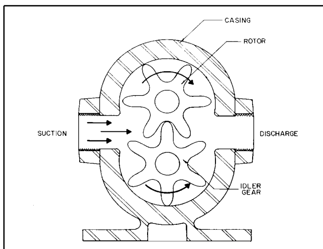
Fig. 5. External gear pump.
