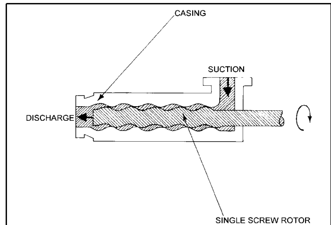
Fig. 8. Single screw pump.
