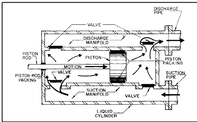
Fig. 2c. Double acting piston pump.
