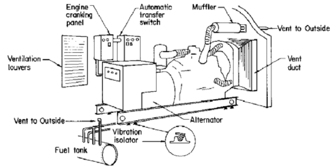
Figure 1. Stationary Standby Power Unit
