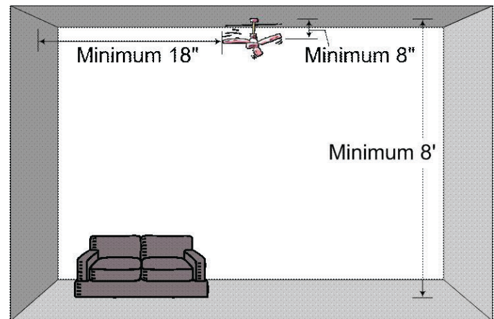
Figure 1. Minimum space requirements for a ceiling fan installation recommended by the US Department of Energy.
