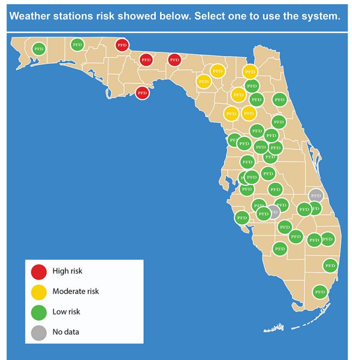
Figure 1. Citrus PFD Advisory System available at http://agroclimate.org/tools/cas .
