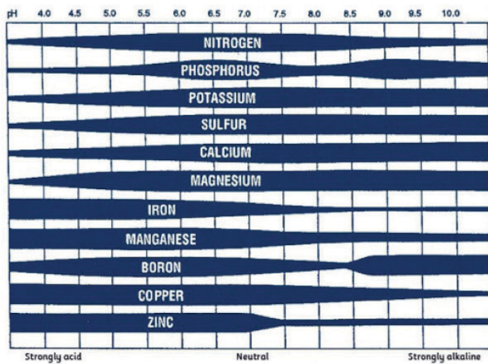
Figure 1. Nutrient availabilities with different soil pH values (Silveira 2013). The width of the blue band illustrates the approximate availability of the specific nutrient. The wider the band, the more available the nutrient is, and the narrower the band, the less available the nutrient is for crop growth.
