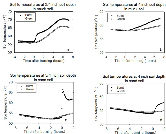
Figure 2. Mean soil temperatures during burning in burnt cane harvested plots, and comparison with concurrently recorded soil temperatures in green cane harvested plots, at 3/4-inch and 4-inch soil depths in muck and sand. Time = 0 = onset of burn event. Credits: Sandhu et al. (2013)
