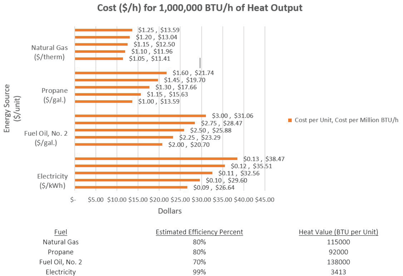
Figure 7. Comparison of fuel costs for equivalent heat output. Credits: J. A. Watson, UF/IFAS
