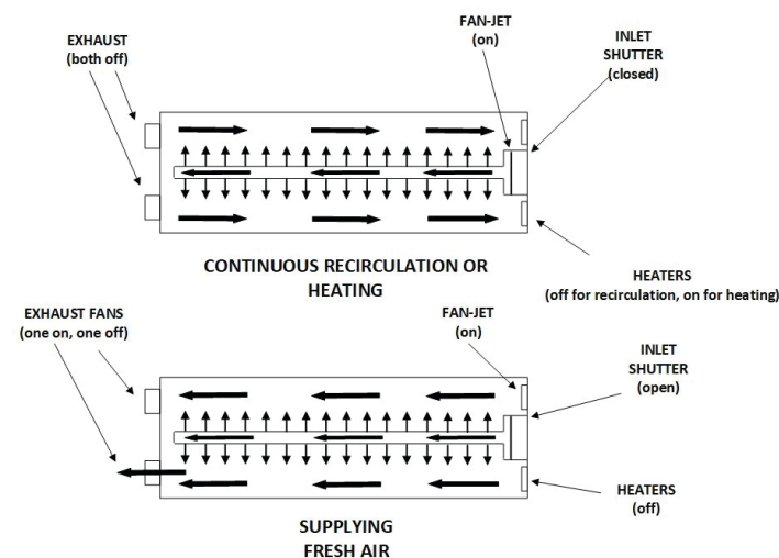
Figure 4. Schematic view of fan-jet poly-tube systems.
