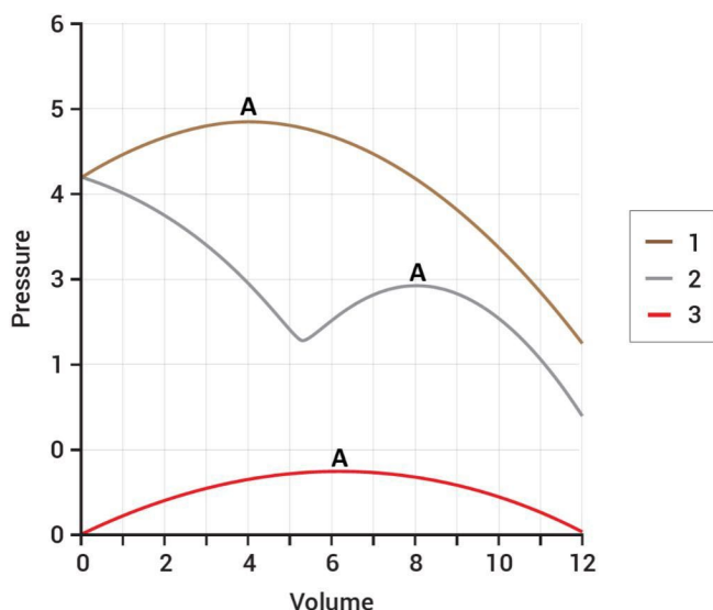
Figure 4. Characteristic curves for centrifugal blower (1), vane-axial fan (2) and propeller fan (3). Point A corresponds to peak pressure points.
