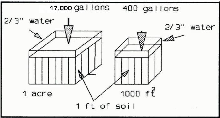
Figure 6. Irrigation volumes required for different size areas to replenish a soil ( 1''/\text{ft} SWHC) depleted to 50% using an impact sprinkler.
