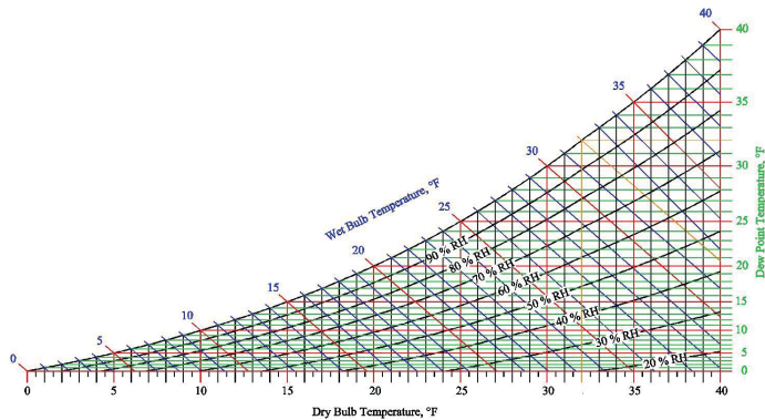
Figure 1. Psychrometric chart.
