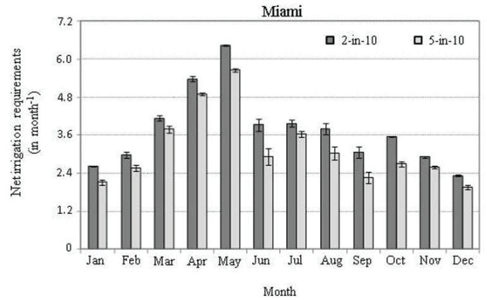
Figure 11. Long-term (1980–2009) mean monthly distribution of the 2-in-10 (80 th percentile) and 5-in-10 (50 th percentile) net irrigation requirements for Miami, FL. Error bars represent the standard deviation due to different root zones and soil types across all time. Credits: C. C. Romero, UF/IFAS
