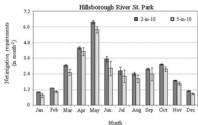
Figure 15. Long-term (1980–2009) mean monthly distribution of the 2-in-10 (80 th percentile) and 5-in-10 (50 th percentile) net irrigation requirements for Hillsborough River State Park, FL. Error bars represent the standard deviation due to different root zones and soil types across all time. Credits: C. C. Romero, UF/IFAS
