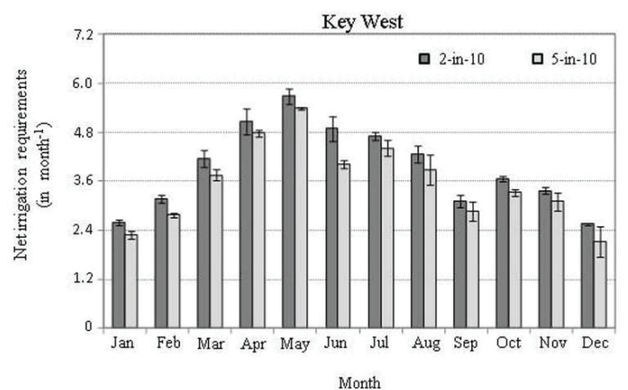
Figure 12. Long-term (1980–2009) mean monthly distribution of the 2-in-10 (80 th percentile) and 5-in-10 (50 th percentile) net irrigation requirements for Key West, FL. Error bars represent the standard deviation due to different root zones and soil types across all time. Credits: C. C. Romero, UF/IFAS
