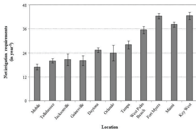
Figure 2. Yearly average net irrigation requirement in all locations in Florida. Error bars represent the standard deviation due to different root zones and soil types across years. Credits: C. C. Romero, UF/IFAS
