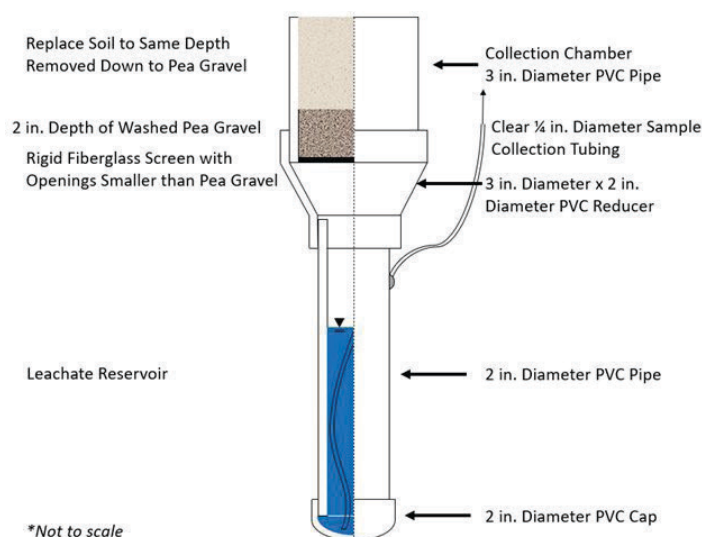
Figure 1. Schematic of lysimeter design showing sizing of different parts.
