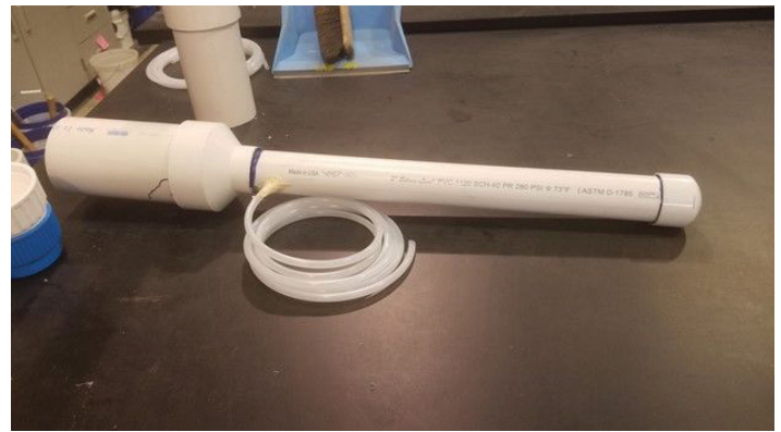
Figure 2. Assembled drainage lysimeter with collection chamber, reducer, reservoir, and purge tube shown.
