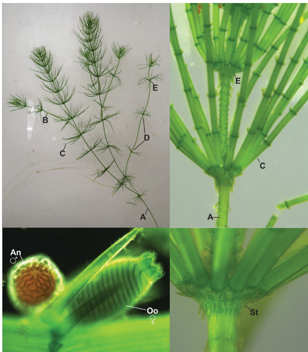
Figure 2. (Top left to right) The basic morphology of Chara , including the main stem or axis (A), branches (B), whorl of branchlets (C), internode (D), and the nodes (E). (Bottom left to right) Male and female reproductive structures in Chara , including the female oogonium (Oo) and the male antheridium (An). Stipulodes (St) morphology is often a method used to identify species.
