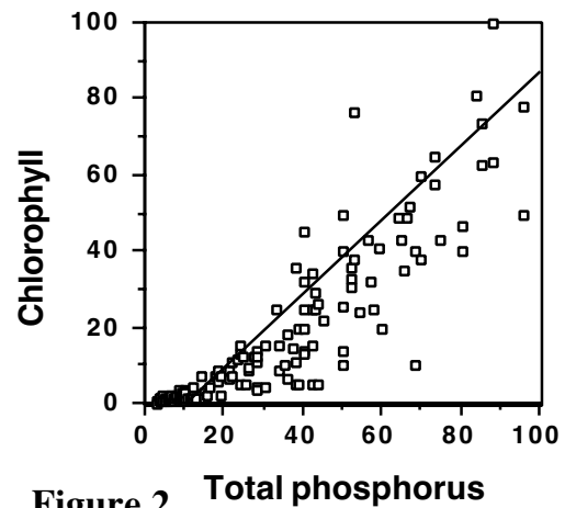
Figure 2. Total phosphorus
