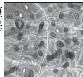
Closterium
