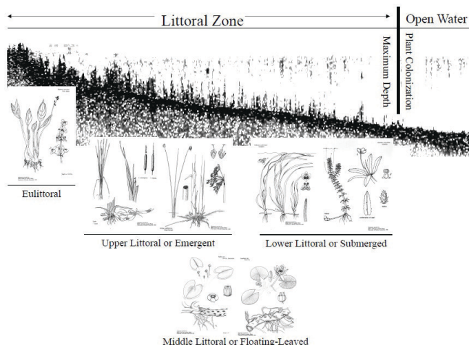
Figure 7. Diagram of a lake's littoral zone.
