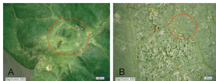
Figure 8. Adult bean thrips, Caliothrips fasciatus Pergande on bean leaf (A) (red circle), and immature stages of Caliothrips fasciatus Pergande, showing first and second instar larva (B) (red circle). In both figures also showing the feeding injury by thrips (white colors and stipples).
