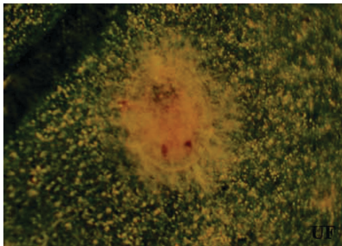
Figure 21. Bemisia tabaci nymph infected with the entomopathogenic fungus, Paecilomyces fumosoroseus .
