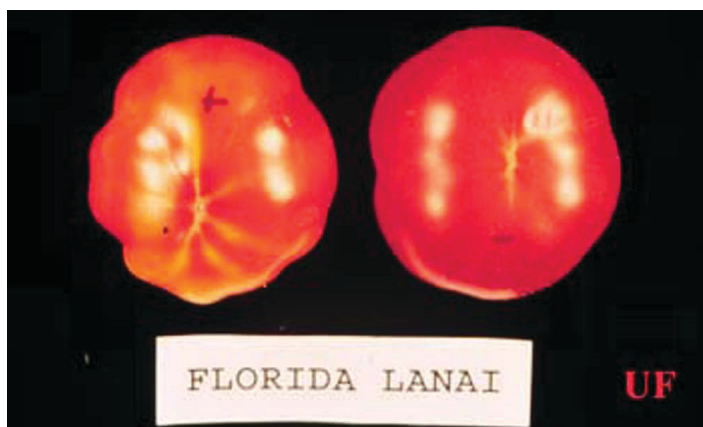
Figure 9. 'Florida Lanai' cherry tomato showing external symptoms of Bemisia -induced tomato irregular ripening disorder (left) and control fruit from uninfested plant (right).
