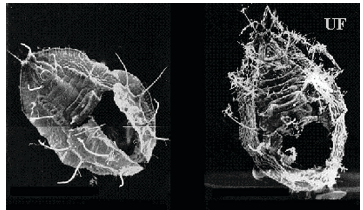
Figure 4. Exuviae of Bemisia with characteristic T-shaped whitefly adult emergence slit (left), and exuviae of Bemisia with round emergence hole through which an adult parasitoid emerged (right).
