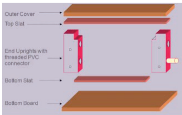
Figure 1. Simple plans for an observation bee hive. More detailed plans can be found at: http://www.mediafire.com/view/mikw31dqdd0jsjh/A_Plan_for_a_Very_Simple_Observation_Hive1.doc Credits: Developed by Jim Tew; used with permission.
