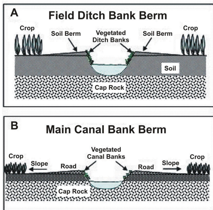
Figure 2. Schematic diagram of A) field ditch berm and B) main canal bank berm.
