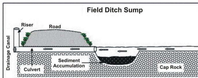
Figure 4. Schematic diagram of field ditch sump.
