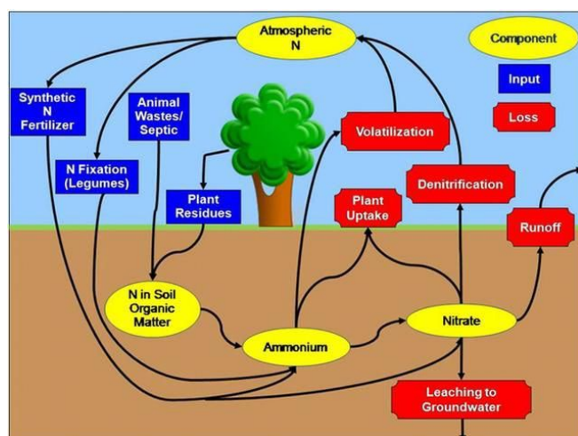
Figure 1. The nitrogen cycle. Credit: UF/IFAS
