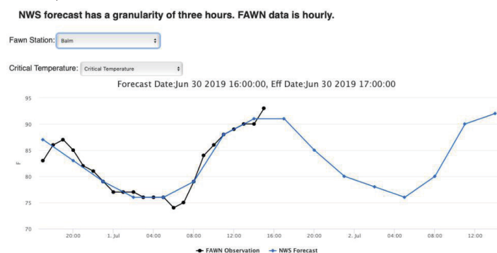
Figure 1. Forecast Tracker
