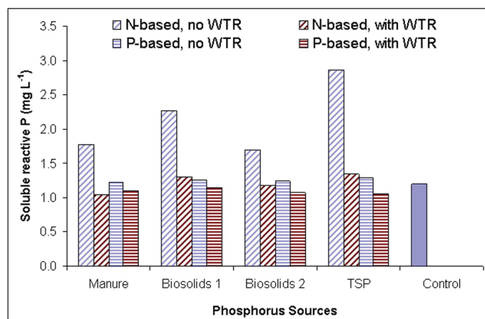
Figure 3. Effects of P sources (applied at N-based- and P-based rates) and WTR amendment (10 tons/acre) on the soluble phosphorus concentrations of shallow (~0.9 m) groundwater samples obtained from a field study.
