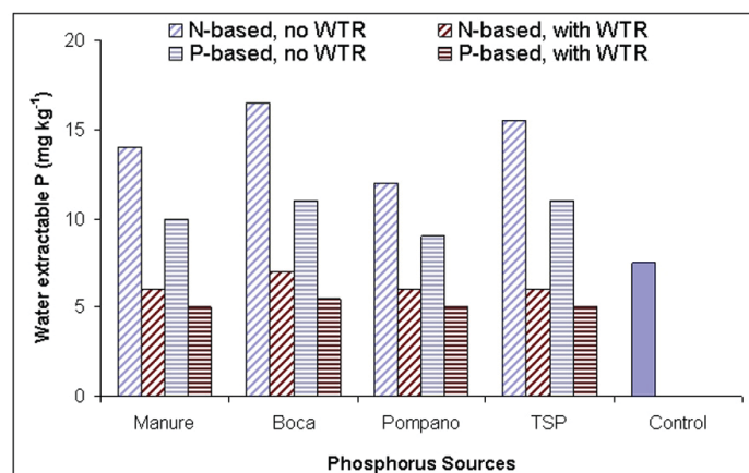
Figure 2. Effect of phosphorus sources (applied at N-based- and P-based rates) and WTR amendment (10 tons/acre) on water extractable phosphorus saturation (WEP) of the A horizon (0-5 cm depth) of the soil samples in a field study.
