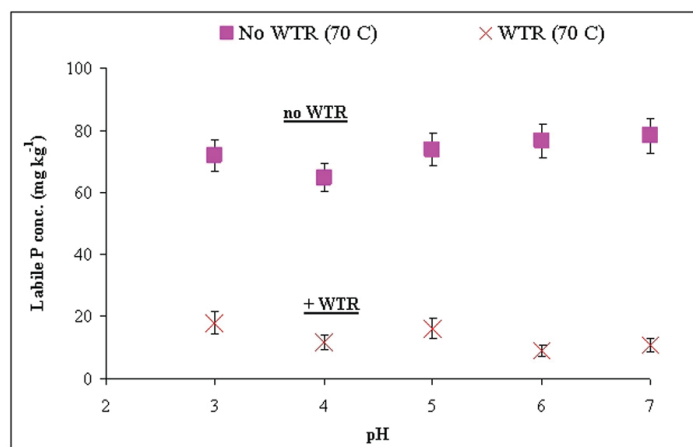
Figure 4. pH effects on labile P of P impacted Immokalee soil samples incubated for 4.5 yr at 70°C. Error bars denote one standard error of the mean.
