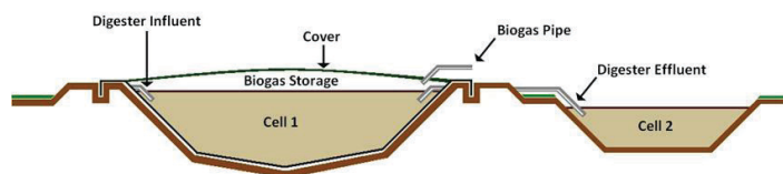
Figure 1. Schematic of a covered anaerobic lagoon digester. Credits: EPA, http://epa.gov/agstar/anaerobic/ad101/anaerobic-digesters.html
