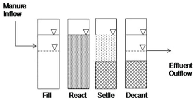
Figure 6. Schematic of a batch digester. Credits: Doug Hamilton, Oklahoma State University
