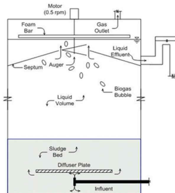
Figure 4. Schematic of an induced blanket digester.
