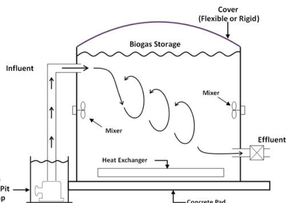
Figure 3. Schematic of a complete mix digester.
