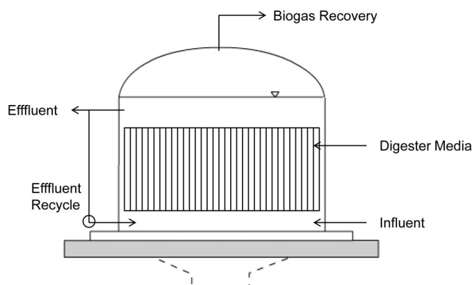
Figure 5. Schematic of a fixed-film digester.
