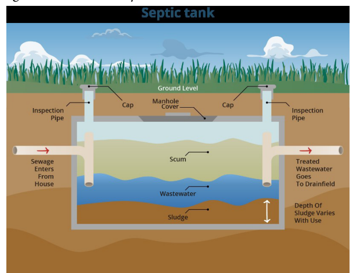
Figure 1. A conventional septic tank.
