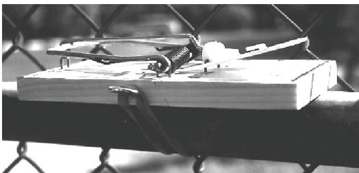
Figure 7. Rat trap secured to the support pipe of a chain link fence showing the use of eye screws and rubber bands to secure the trap without slipping.
