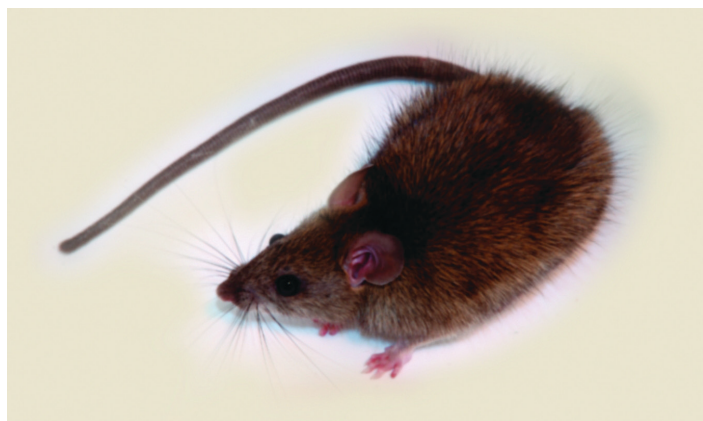
Figure 2. Roof rat.
