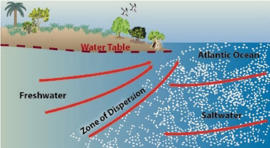
Figure 12. Saltwater intrusion into coastal aquifers. Credits: P. Fletcher, adapted from USGS
