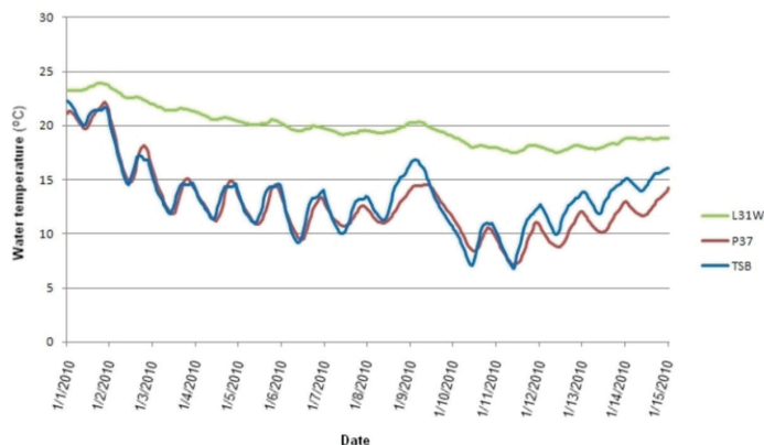
Figure 6. Water temperatures at three hydrostations in Everglades National Park during record cold spell.
