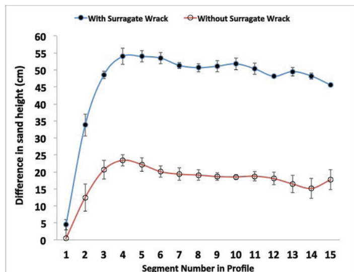
Figure 8. Relative sand height ( \pm 1 standard error, n=6 ) (cm) 2 years after planting (May 2010 - August 2012) by 60 cm segments across Uniola paniculata (sea oats) plantings with surrogate wrack (8 inches of wheat straw mulch) or without surrogate wrack; segment 1 was outside the plot area and represents bare sand with no sea oats. Credits: Debbie Miller, UF/IFAS
