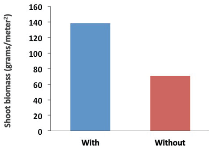
Figure 5. Shoot biomass (g/m 2 ) of Uniola paniculata (sea oats) two years after planting with and without surrogate wrack. Credits: Debbie Miller, UF/IFAS
