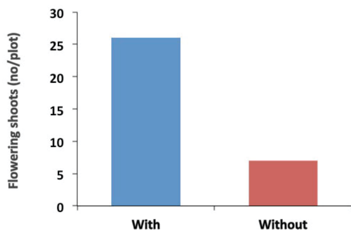
Figure 6. Number of flowering shoots of Uniola paniculata (sea oats) per plot with and without surrogate wrack two years after planting. Credits: Debbie Miller, UF/IFAS
