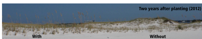
Figure 7. Sand accumulation and presence of sea oats flowering shoots two years after planting with and without surrogate wrack. Credits: Sean Claypool, UF/IFAS
