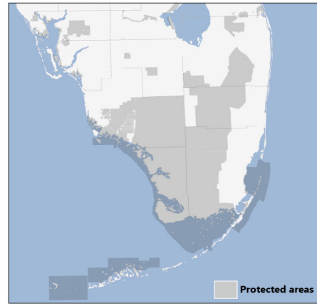
2060 Climate suitability for the Cape Sable seaside sparrow.
