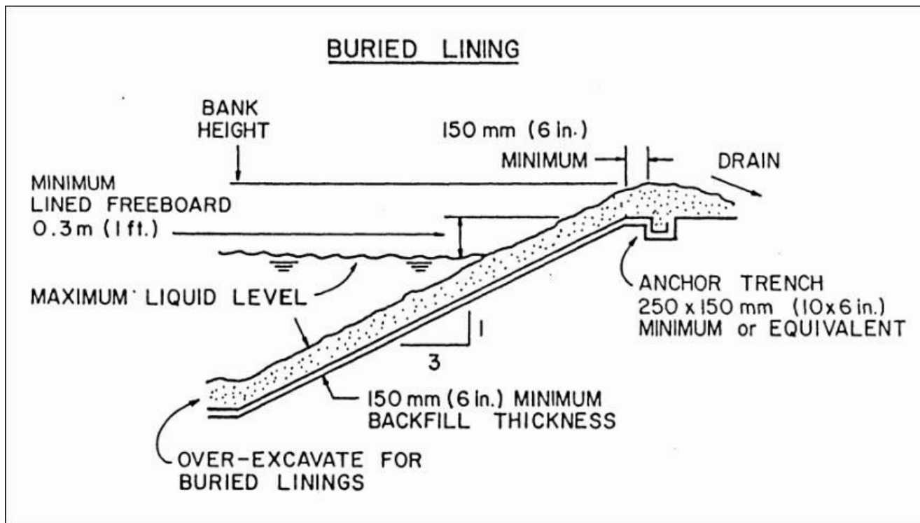
Figure 3. Placement of anchor trench for buried lining.
