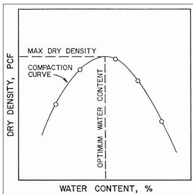
Figure 1. Compaction curve.
