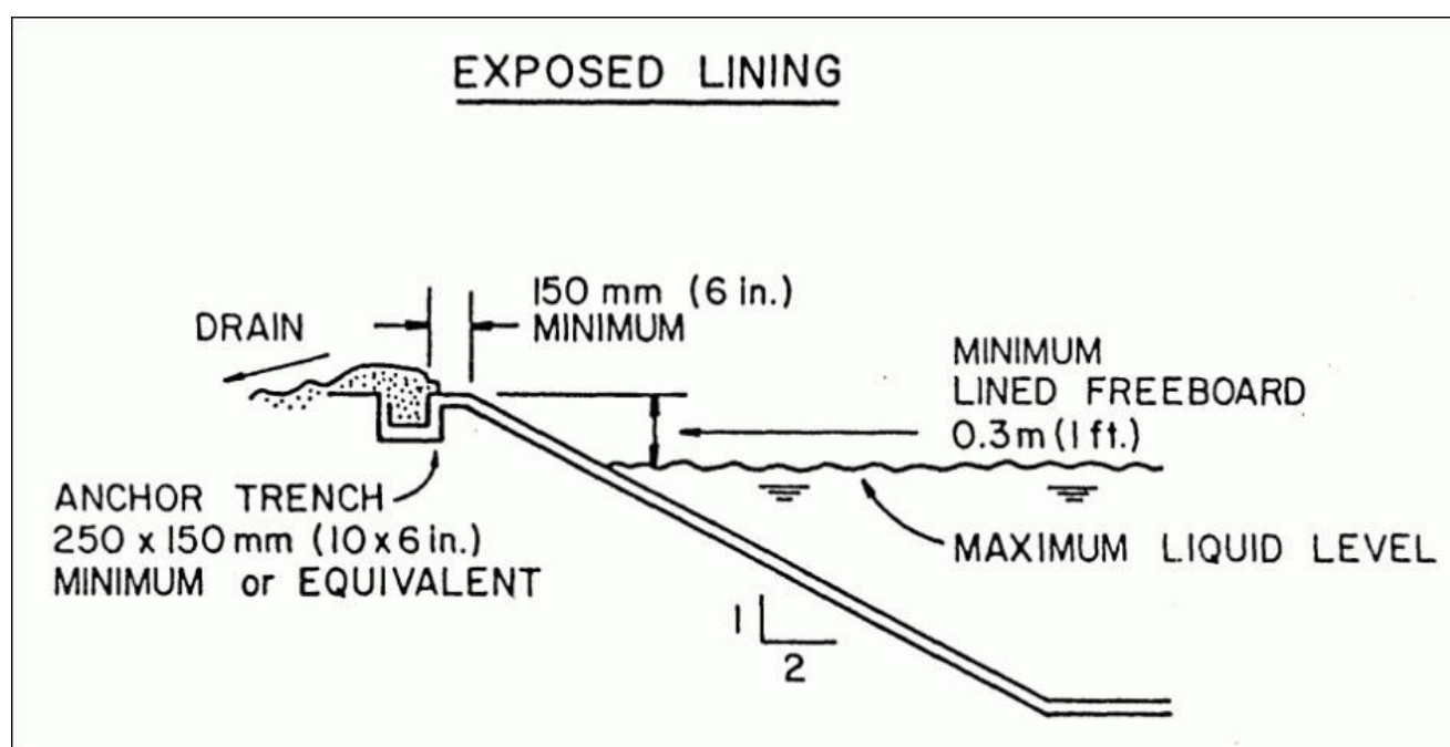
Figure 2. Placement of anchor trench for exposed lining.
